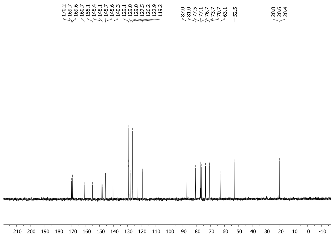
Figure S2: ^{13}\text{C} -NMR (75.5 MHz, \text{CDCl}_3 ) spectrum.
