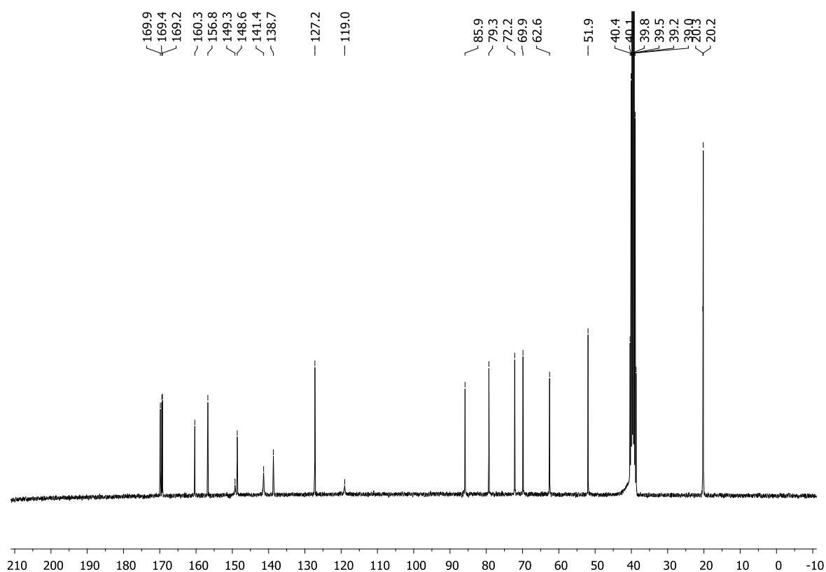
Figure S8: 13 C-NMR (75.5 MHz, DMSO-d 6 ) spectrum.
