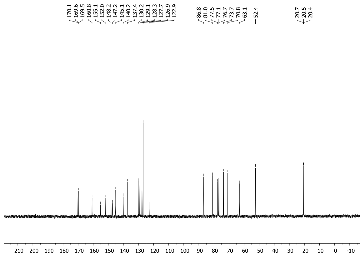
Figure S4: 13 C-NMR (75.5 MHz, CDCl 3 ) spectrum.
