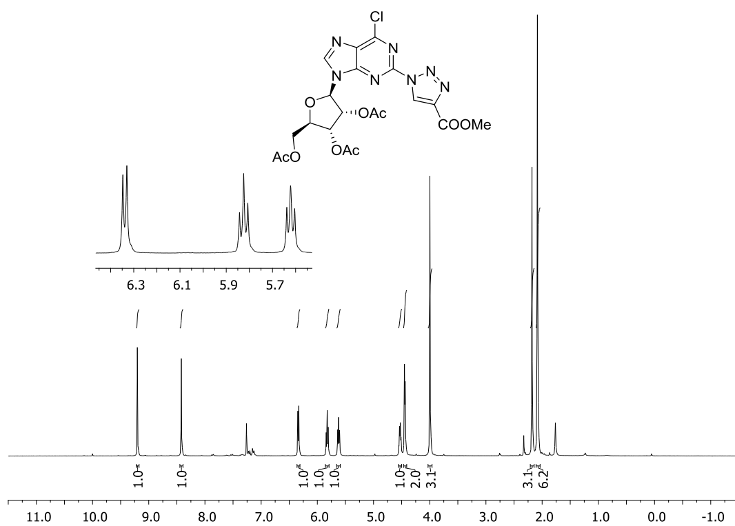
Figure S9: ^1\text{H-NMR} (300 MHz, \text{CDCl}_3 ) spectrum.
