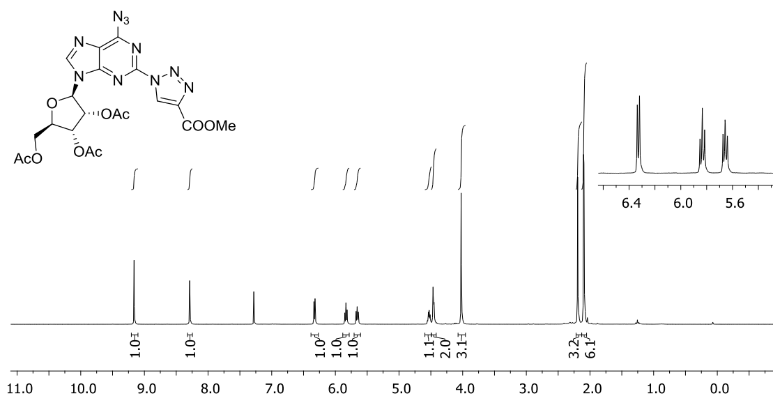
Figure S5: ^1\text{H-NMR} (300 MHz, \text{CDCl}_3 ) spectrum.
