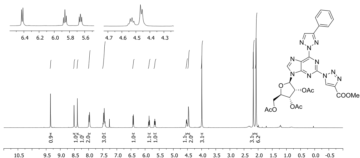
Figure S3: 1 H-NMR (300 MHz, CDCl 3 ) spectrum.
