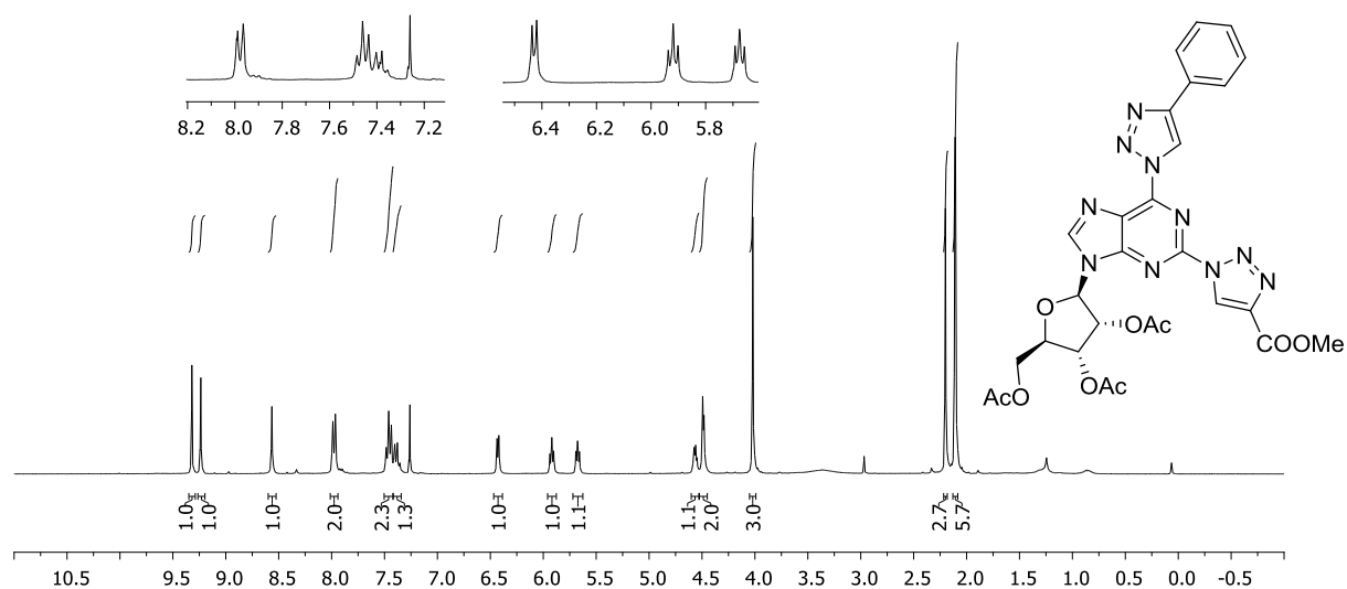
Figure S1: ^1\text{H} -NMR (300 MHz, \text{CDCl}_3 ) spectrum.
