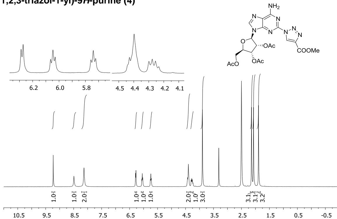
Figure S7: 1 H-NMR (300 MHz, DMSO-d 6 ) spectrum.
