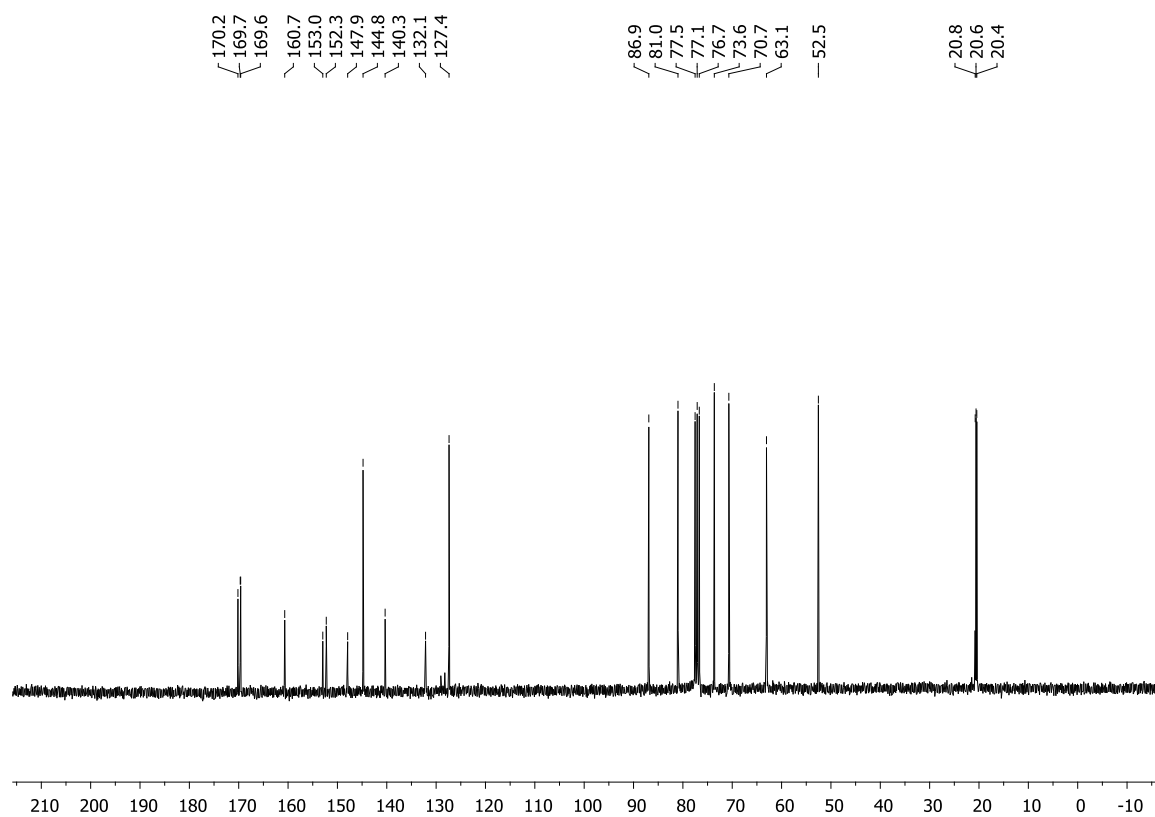
Figure S10: ^{13}\text{C-NMR} (75.5 MHz, \text{CDCl}_3 ) spectrum.
