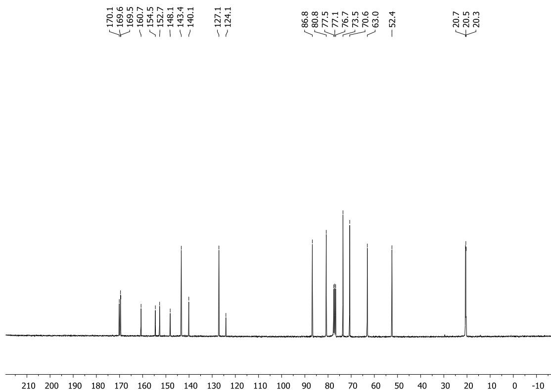
Figure S6: ^{13}\text{C-NMR} (75.5 MHz, \text{CDCl}_3 ) spectrum.
