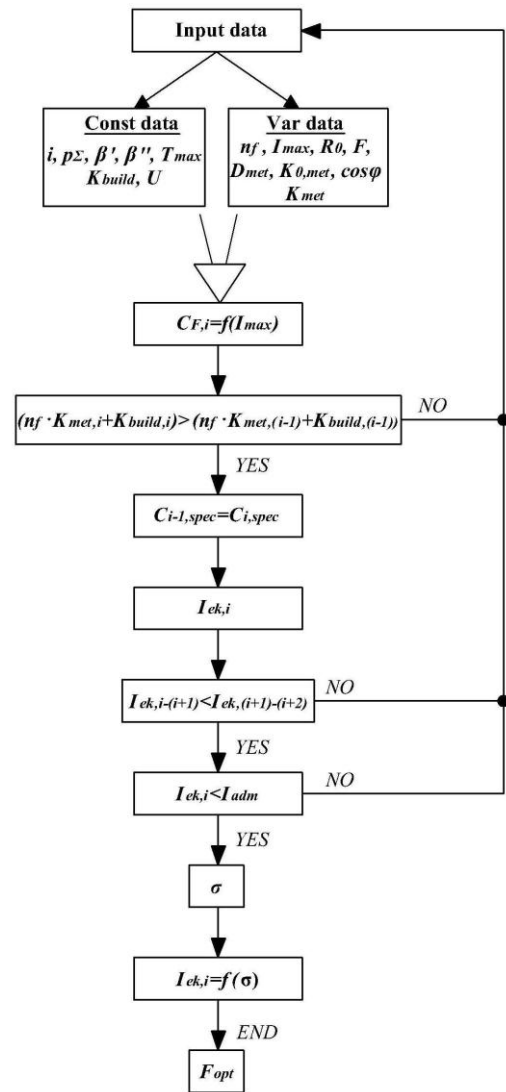
Fig. 9. Algorithm of optimal cross section choice by economic intervals method.
