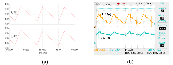
Fig. 16. Simulated (a) and measured current waveforms of inductors L_2 and L_4 (b), D_S = 0.25 .
