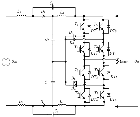
Fig. 2. Three-level NPC quasi-impedance-source inverter.
