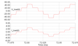
Fig. 8. Output voltage and current of a single-phase three-level NPC qZS inverter.
