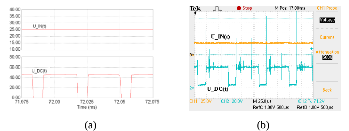
Fig. 17. Simulated (a) and measured waveforms of the input- and the DC-link voltage of a single-phase three-level NPC qZSI (b), D_S = 0.25 .
