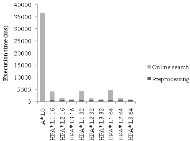
Fig. 7. Pathfinding results in a 1024x1024 node grid
