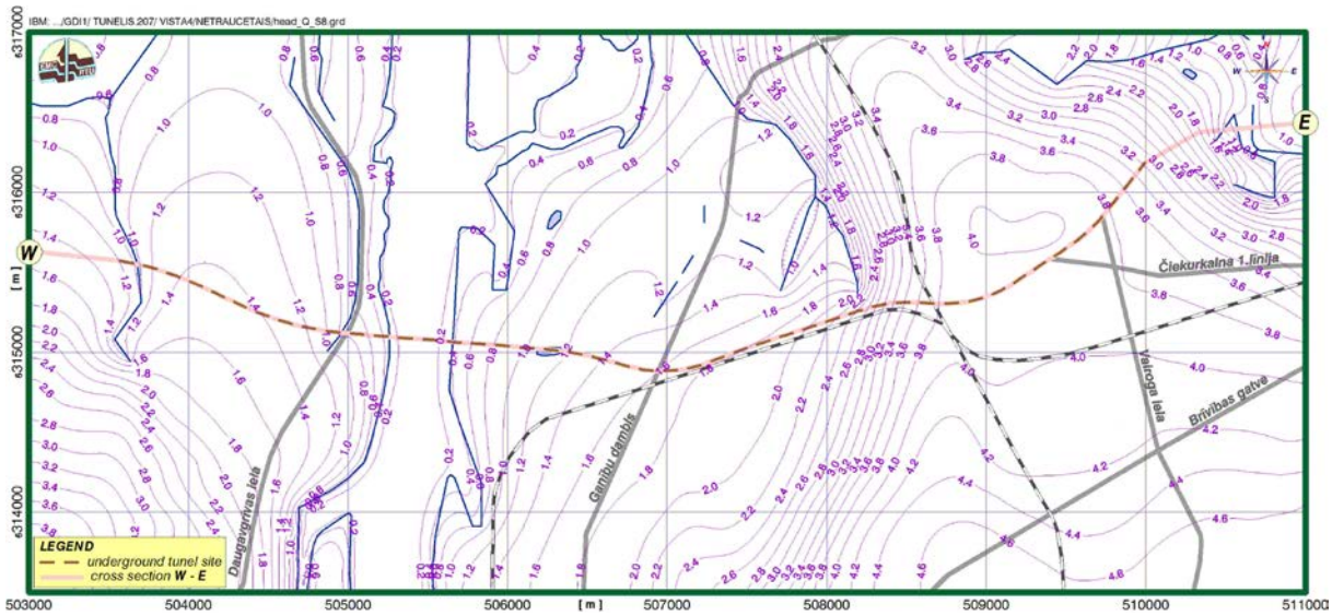
Fig. 5 Head distribution [m asl] of the Q aquifer. To account for the tunnel geometry, the Q aquifer is divided into four parts (Table 1): above tunnel ( Q_1 ), tunnel body ( Q_2 ), below tunnel ( Q_3 ), coarse sand layer ( Q_4 ). It is shown in Fig.4, how the parts Q_1 , Q_2 , Q_3 are used, to approximate the two tunnel drives.
