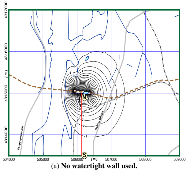
Fig. 8 Depression dt [m] caused by the construction trench.
