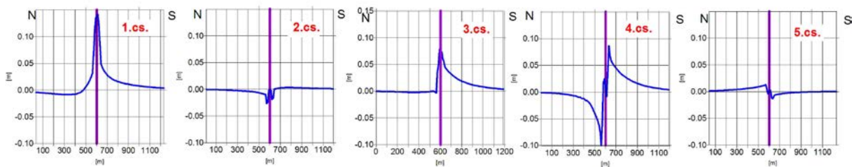
(b) In cross sections orthogonal to tunnel axis.
