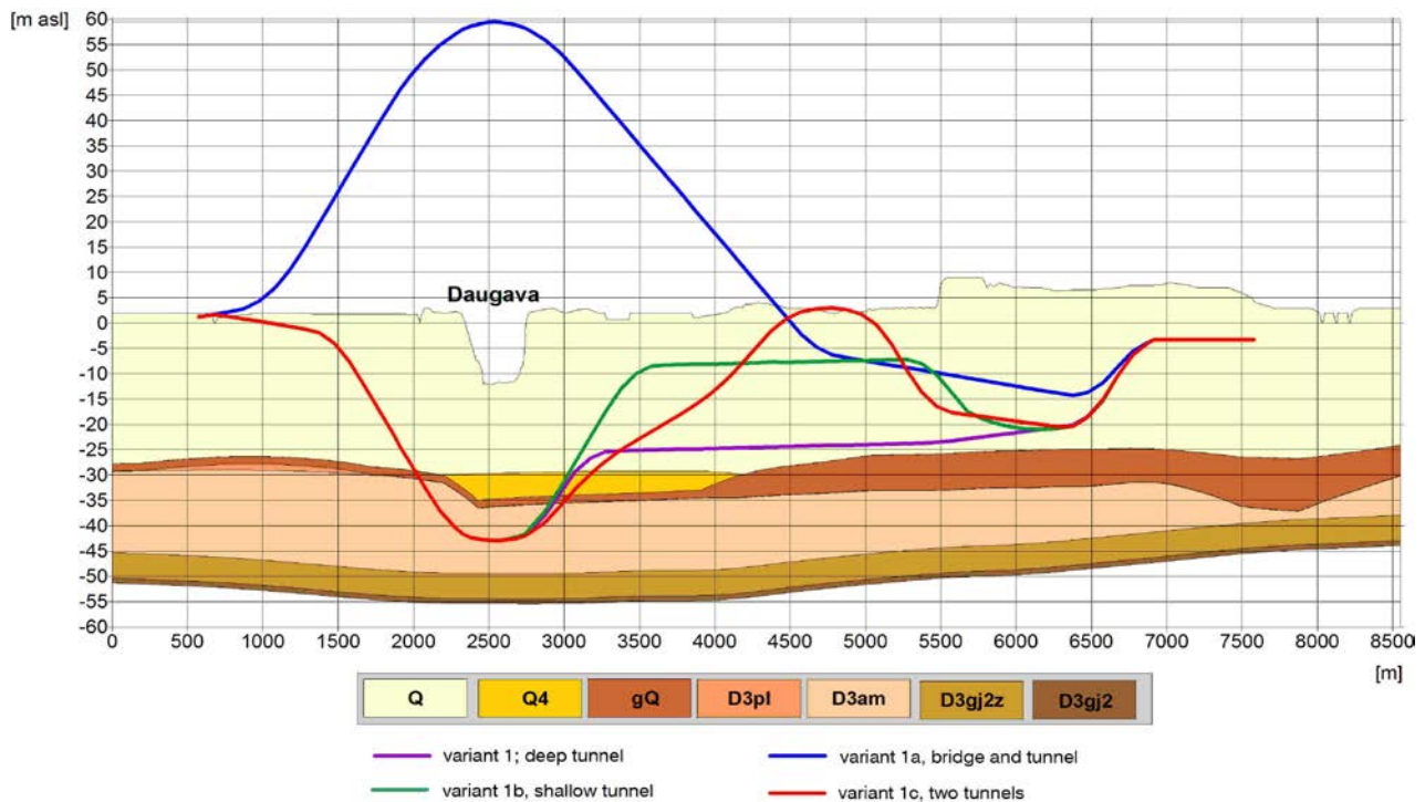
Fig.3 Cross section WE. Variants of tunnel road base.
