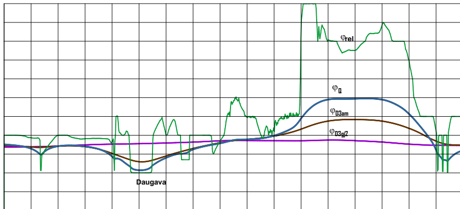
Fig. 6 Cross section WE. Graphs of ground surface \phi_{rel} and heads \phi_Q , \phi_{D3am} , \phi_{D3g2} are shown.
