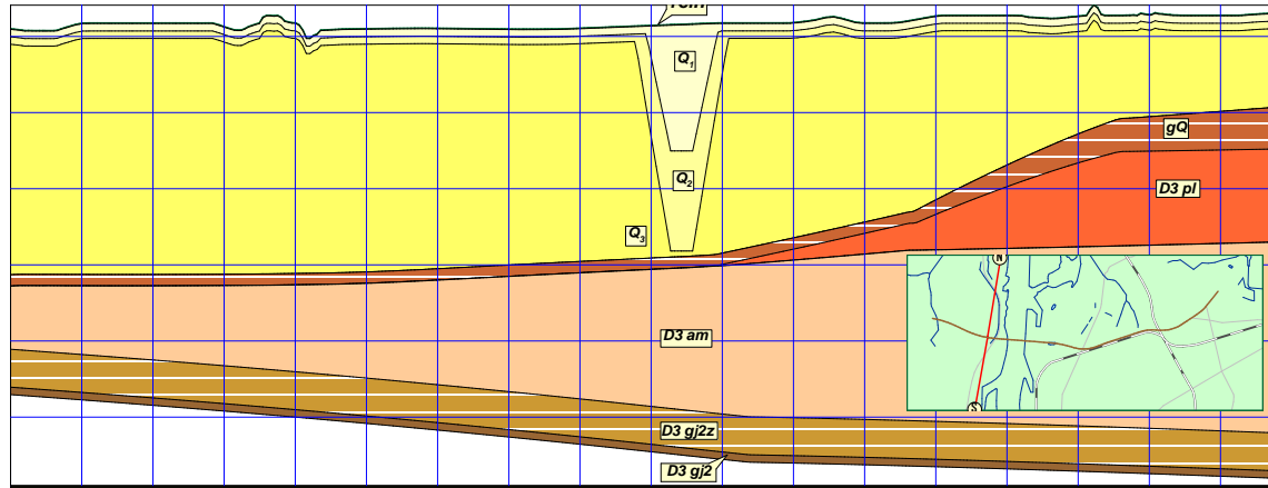
Fig. 4 Cross section NS. Approximation of tunnel system and its surroundings.
