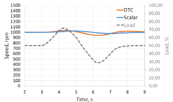
Fig. 13. Drive speed response on variable load of sinusoidal profile.
