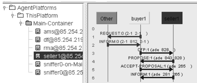
Fig. 5. Agent system with two agents and a common ontology.
