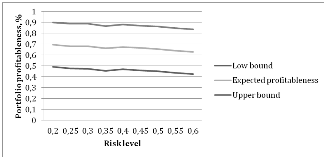
Fig. 2. The dependence of expected portfolio profitableness on risk level.
