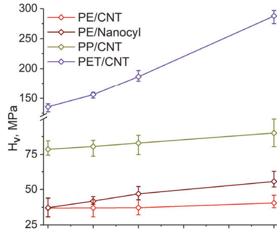
Fig. 12. Polymer/CNT nanocomposite H_V dependence on CNT concentration.
