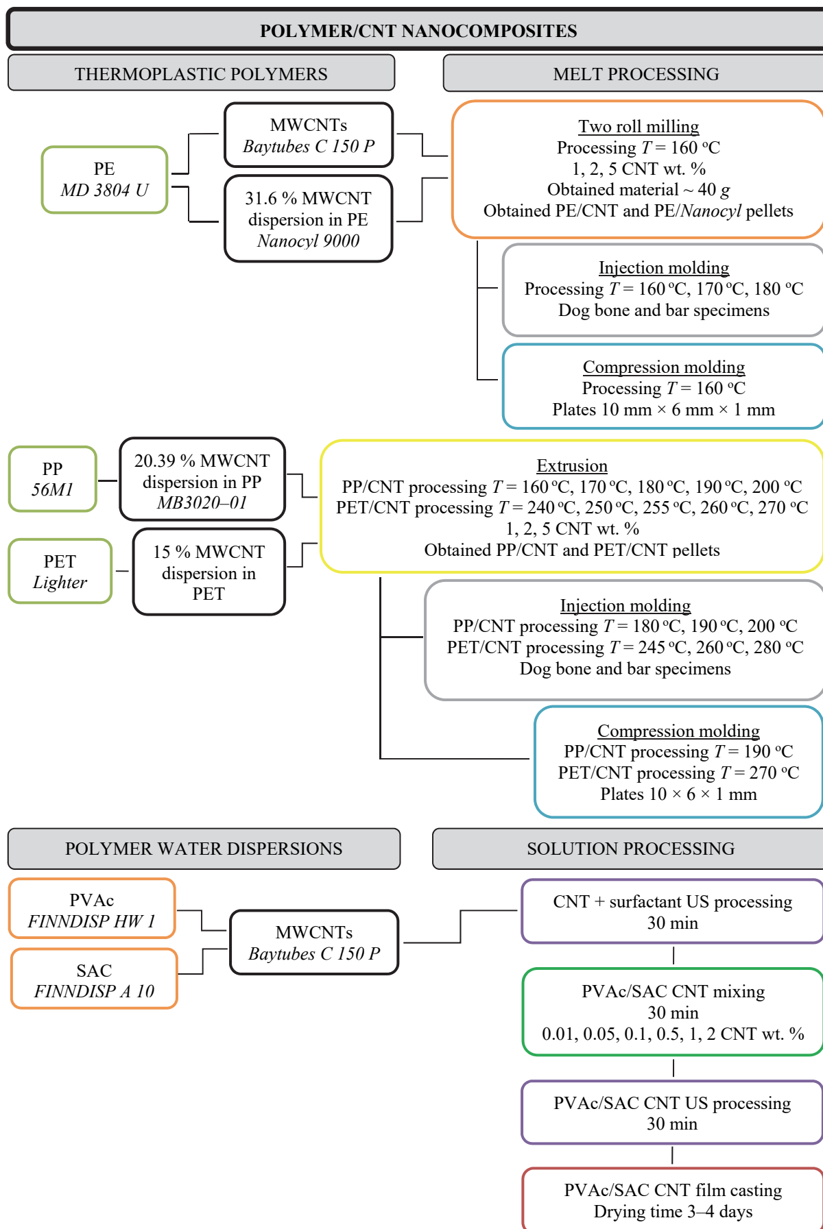
Fig. 1. Polymer nanocomposite processing scheme.
