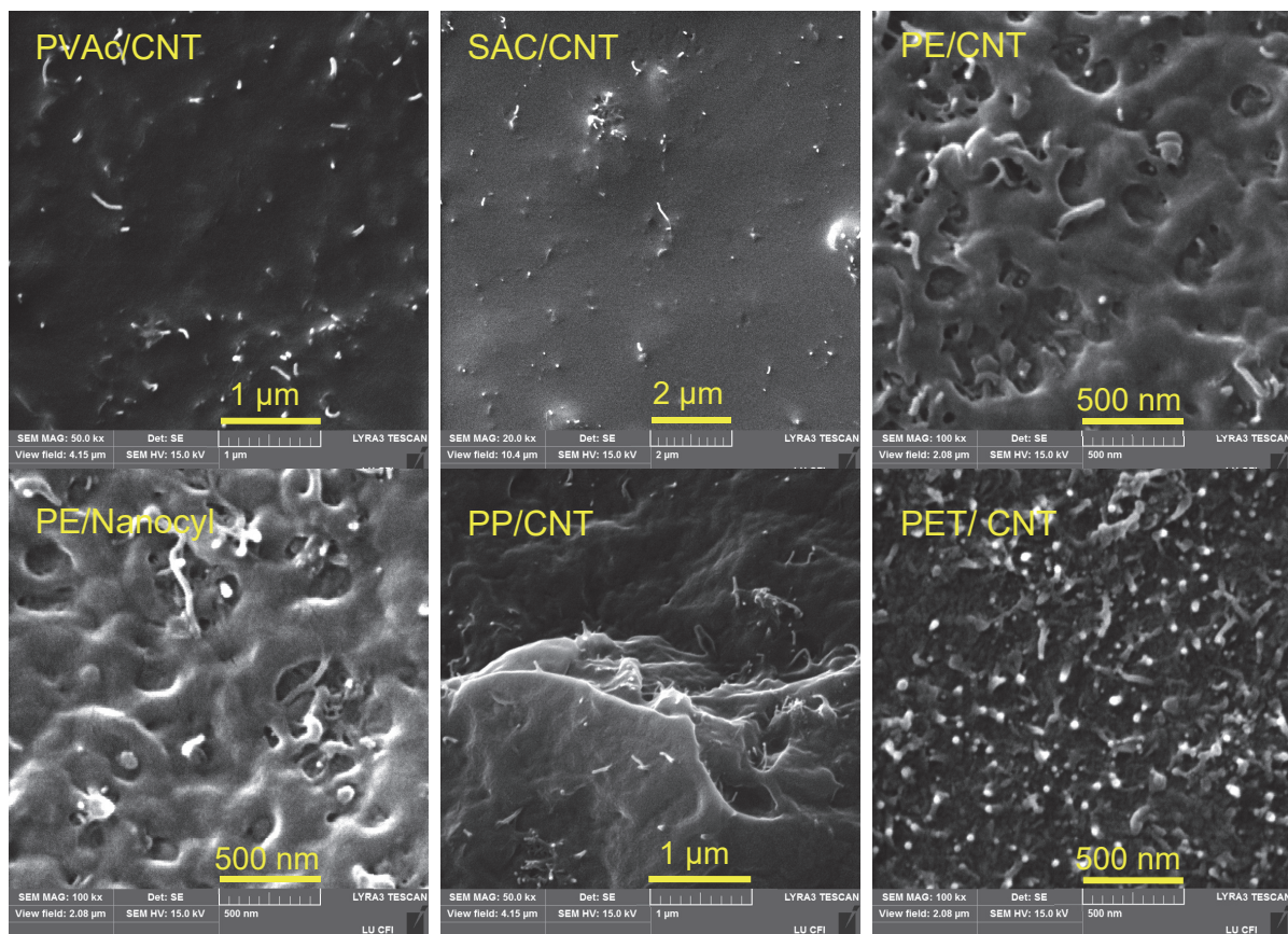
Fig. 3. SEM microphotographs of polymer/CNT nanocomposites.
