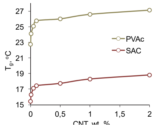
Fig. 15. Changes in PVAc/CNT and SAC/CNT nanocomposite T_g .
