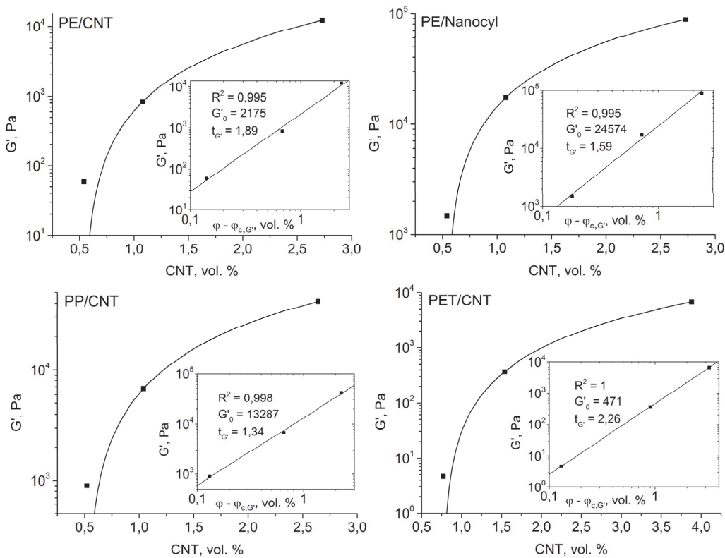
Fig. 21. Polymer nanocomposite rheological percolation parameters.
