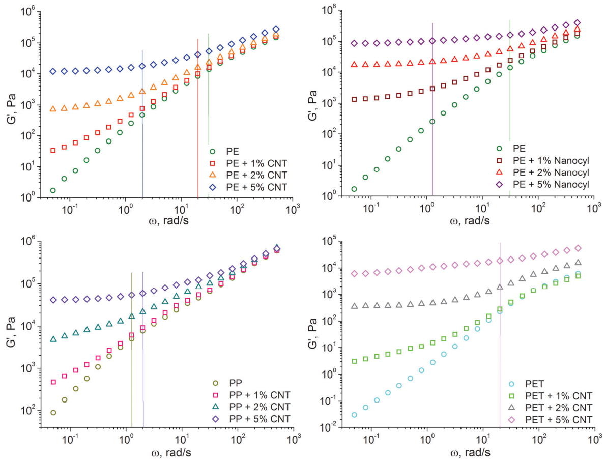
Fig. 21. Polymer/CNT nanocomposite storage modulus G'(\omega) curves.
