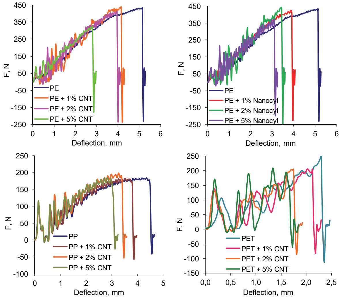
Fig. 14. Polymer/CNT nanocomposite impact force curves.
