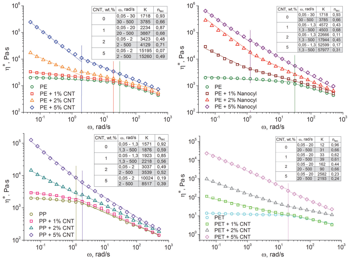
Fig. 20. Polymer/CNT nanocomposite complex viscosity \eta^*(\omega) curves.
