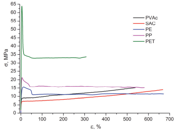
Fig. 5. Polymer matrix tensile \sigma(\epsilon) curves.
