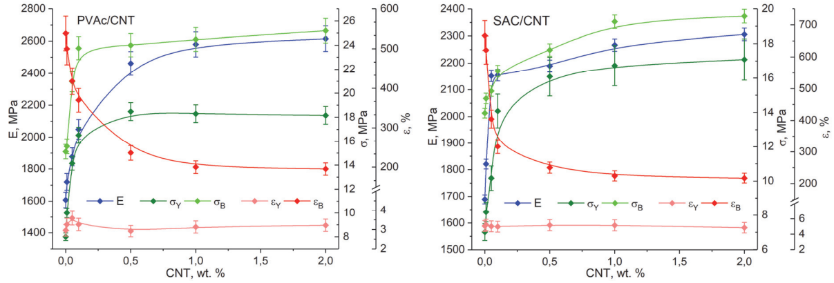
Fig. 6. PVAc/CNT and SAC/CNT nanocomposite tensile parameter E , \sigma_Y , \sigma_B , \varepsilon_Y and \varepsilon_B dependence on CNT concentration.
