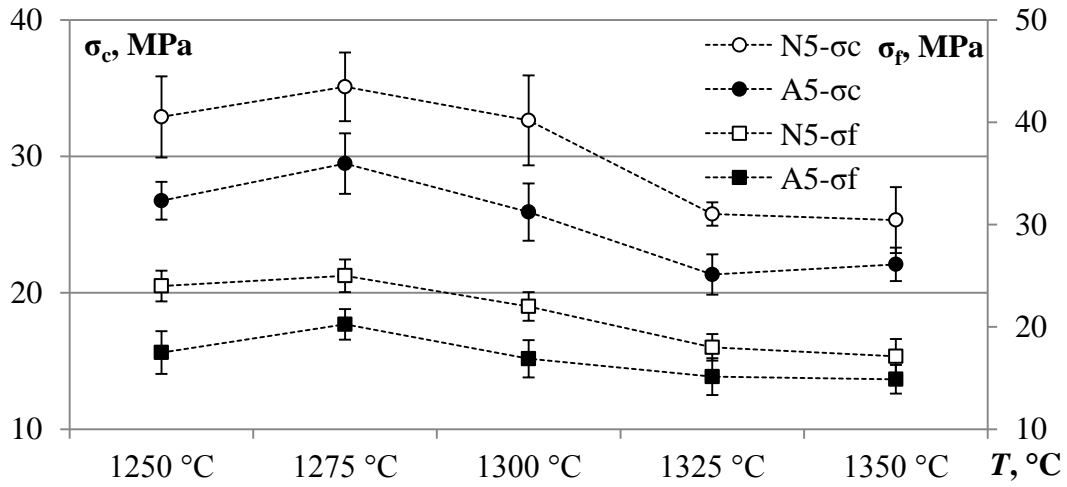
Fig. 3.11. Compressive ( \sigma_c ) and flexural ( \sigma_f ) strength of samples A5 (●, ■) and N5 (○, □) depending on firing temperature (T).
