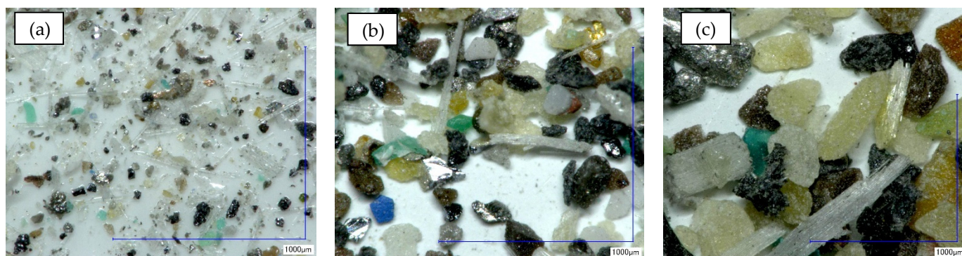
Figure 4. Optical images at magnification \times 200 times, of disintegrator-crushed PCBs fractions: (a) is d < 90 \mu\text{m} ; (b) is d = 90\text{--}180 \mu\text{m} ; and (c) is d = 180\text{--}350 \mu\text{m} and designated [A], [B] and [C], respectively.
