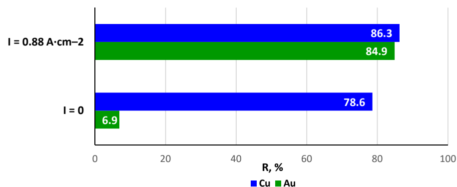
Figure 10. Effect of AC applying on gold and copper leaching degree. Experimental conditions: Raw material—fraction [A], t_{\text{ex}} = 2 \text{ h} , S/L = 8.6 \text{ g} \cdot \text{L}^{-1} , and C_{\text{HCl}} = 6 \text{ M} .
