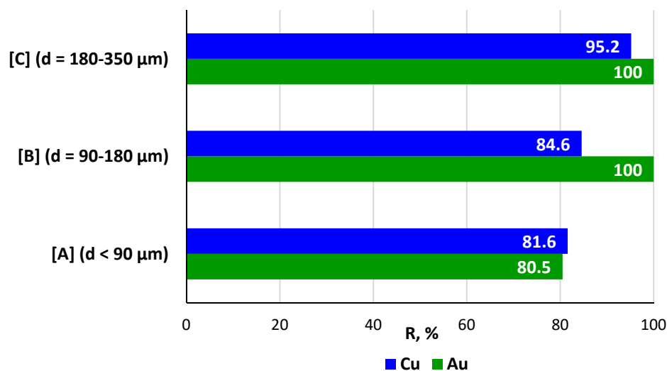
Figure 9. Impact of raw material particle size on the degree of gold and copper leaching. Experimental conditions: i = 0.66 \text{ A} \cdot \text{cm}^{-2} , t_{\text{ex}} = 2 \text{ h} , S/L = 8.6 \text{ g} \cdot \text{L}^{-1} , and C_{\text{HCl}} = 6 \text{ M} .
