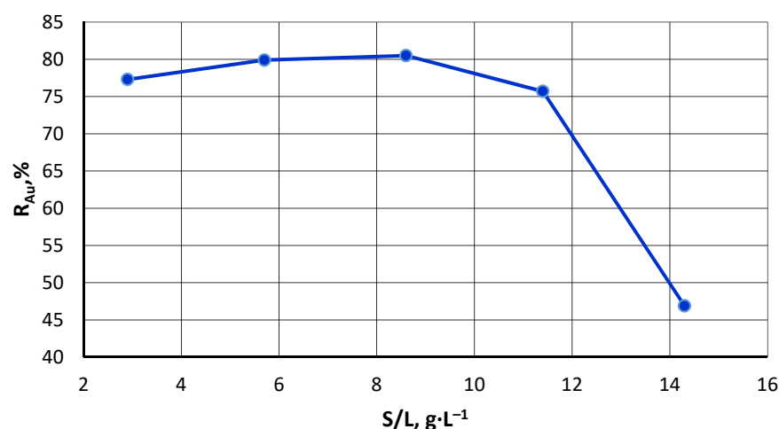
Figure 8. Impact of S/L ratio on the degree of gold leaching. Experimental conditions: Raw material fraction [A], C_{\text{HCl}} = 6 \text{ M} , i = 0.66 \text{ A} \cdot \text{cm}^{-2} , and t_{\text{ex}} = 2 \text{ h} .
