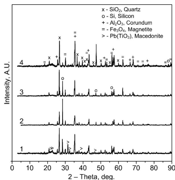
Figure 14. XRD patterns of solid residues from the experiments at different experiment durations: 1–0.5 h, 2–2 h, 3–4 h and 4–5 h. Other experimental conditions are provided in the caption of Figure 13.
