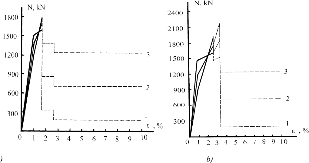
a) b) Fig. 3. Strain of hybrid composite cable a) on the base of steel, GFRP and CFRP and b) on the base of steel, GFRP and Vectran \varepsilon vs. the force N , acting in the cable: 1,2,3 – the dependences, which were obtained at volume fractions of steel, equal to 0.1; 0.4; 0.7, respectively; (—) – stage, when all the components of the cables work commonly; (-----) – stage, when some components are disrupted.
