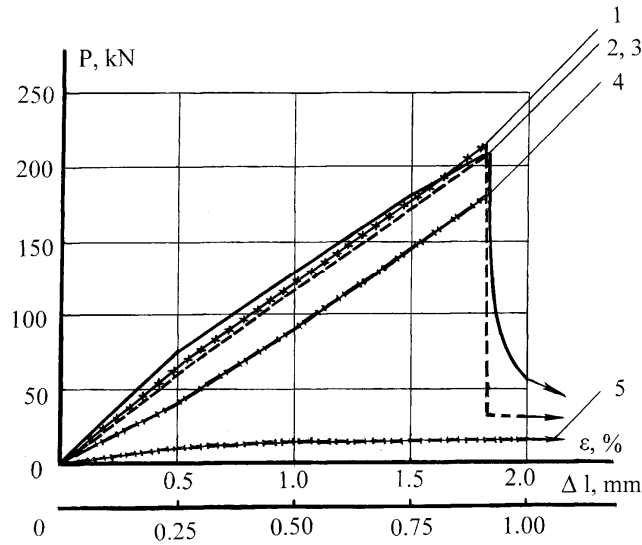
Fig.2. Behaviours of hybrid composite cable: 1 – graph, which was obtained analytically for the composite material on the base of one CFRP tape and two steel tapes with taking into account of two layers of epoxy glue with thickness in 1 mm.; 2 – graph, which was obtained by the experiment for the composite material on the base of one CFRP tape and two steel tapes; 3 – graph, which was obtained analytically for the composite material on the base of one CFRP tape and two steel tapes. Two layers of epoxy glue with thickness in 1 mm were not tacked into account; 4 – graph, which was obtained by the experiment for the CFRP tape; 5 – graph, which was obtained by the experiment for the steel tape. The results were obtained by the strain-measuring device with the length of the base 50 mm.
