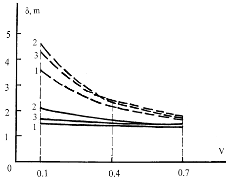
Fig. 4. Dependence of the maximum vertical displacements of the cable roof \delta on the volume fraction of steel in hybrid composite cables V : 1 – variant on the base of steel, GFRP and CFRP; 2 – variant on the base of steel, GFRP and Vectran; 3 – variant on the base of steel, Vectran and CFRP; (—) – stage, when all the components of the cables work commonly; (-----) – stage, when all the components, excluding the steel, are disrupted.
