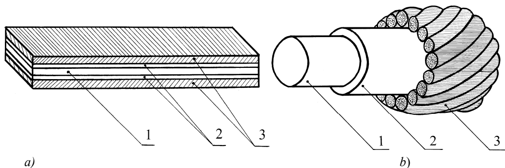
Fig. 1. Hybrid composite elements on the base of steel and FRP; 1 – FRP core; 2 – glue or FRP distributional layer; 3 – steel component.
