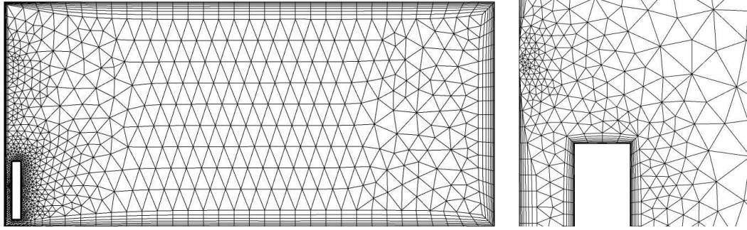
Fig. 2. Typical meshes for the modelled room in the middle cross-section and near the heater.
