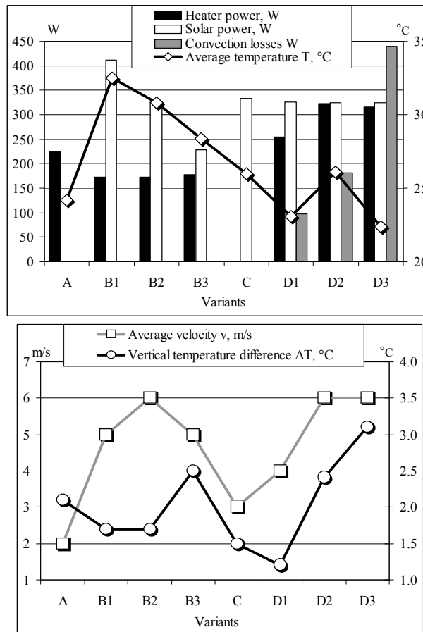
Fig. 3. Heating powers, convection losses, average temperature in the room, vertical temperature difference and airflow velocity in the middle of the room for different variants.
