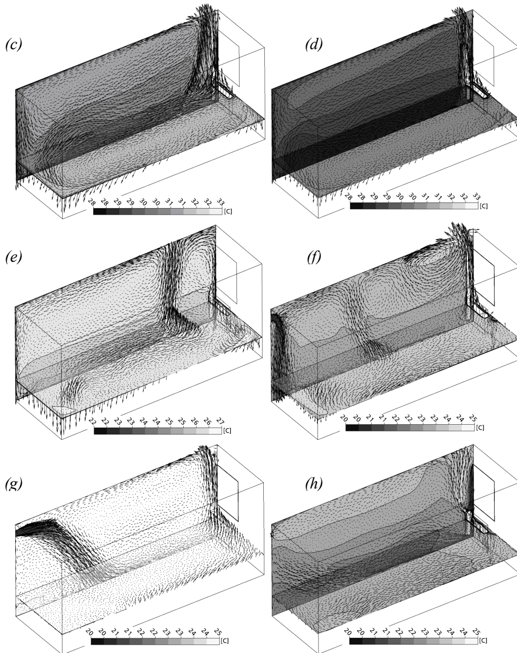
Fig. 4. Velocity vector field and temperature contours in middle vertical cross-section and 0.5m height horizontal cross-section for variants A (a),B1-B3 (b-d),C (e) and D1-D3 (f-h).
