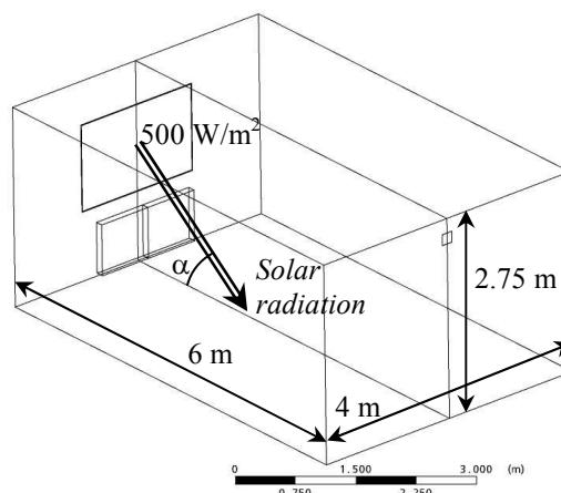
Fig. 1. Layout of a modelled room.
