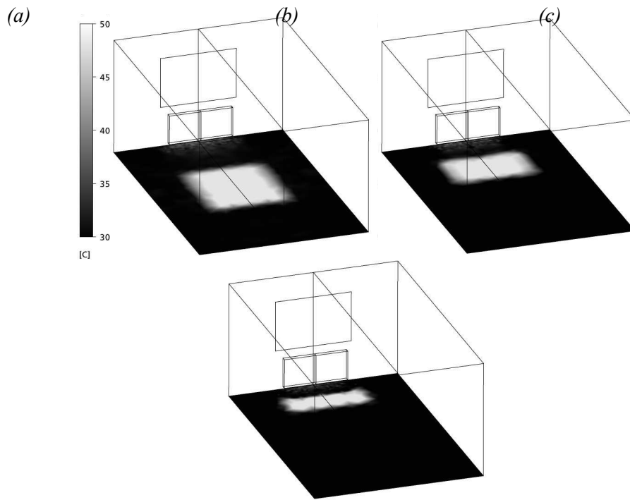
Fig. 5. Temperature distribution on the floor for variants B1 (a), B2 (b) and B3(c).
