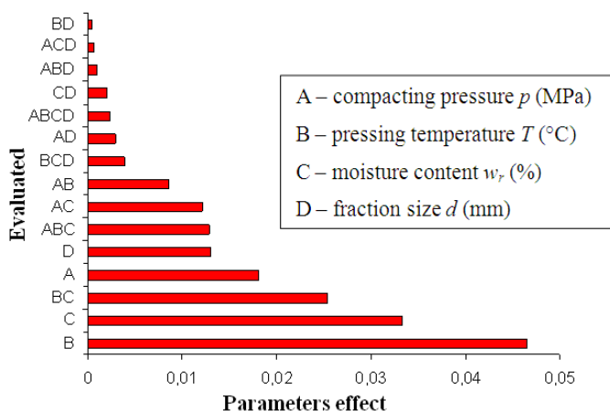
Fig.9 Influence of parameters and their mutual interactions at briquetting process [7]
