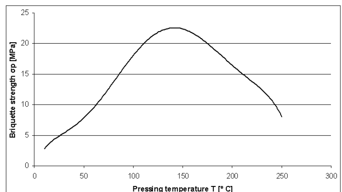
Fig.6 Dependence of briquette strength on pressing temperature [8]
