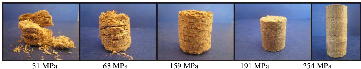
Fig.4 The effect of the compacting pressure to briquette quality [7]
