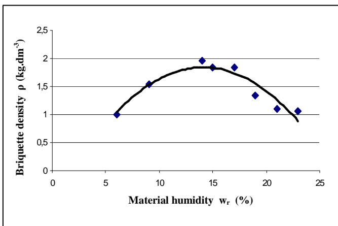
Fig.8 Dependence of the briquette density on material moisture content [8]
