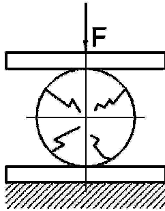
Fig. 3 Testing of briquette compression strength in cleft failure conditions
