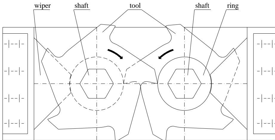
Fig. 1 Principal scheme of two-shaft shredder
