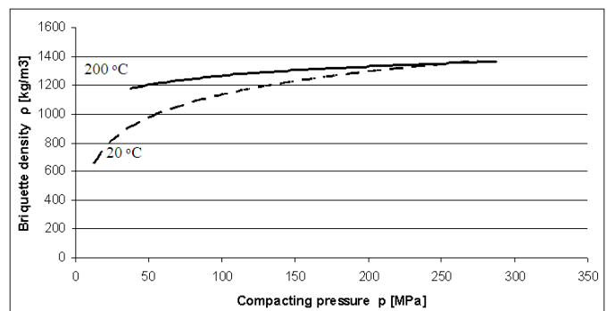
Fig.7 Dependence of briquette density on compacting pressure at various temperatures [8]
