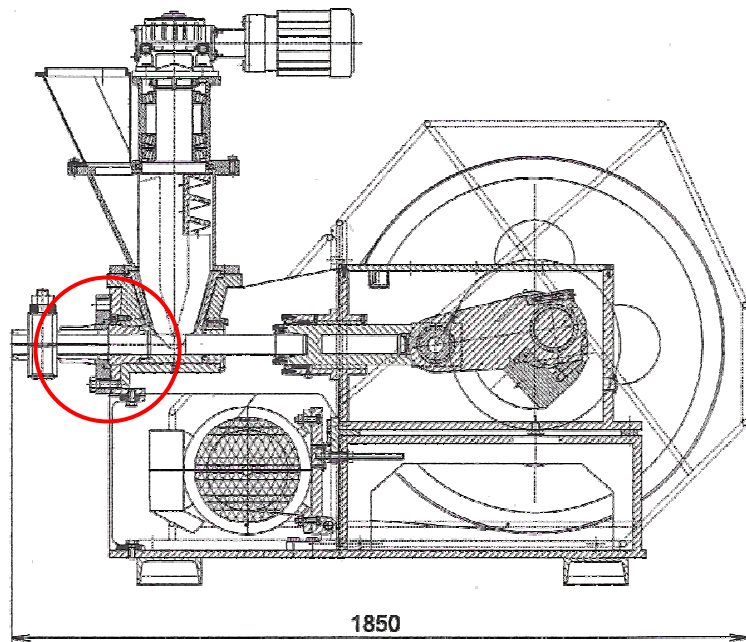
Fig.2 Mechanical (cranked) briquetting press [7]
