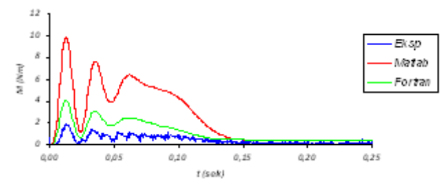
Fig.10. Electromagnetic torque at no-load
