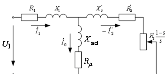
Fig.1. Equivalent circuit diagram of induction motor.
