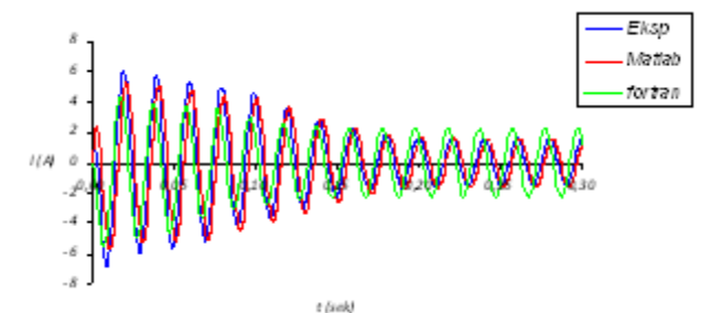
Fig.11. Stator current at full load
