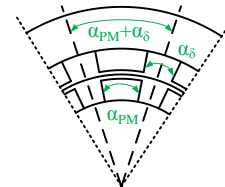
Fig. 3. The definition of PM's angle and angle of airgap. \alpha_{PM} – angle of PM; \alpha_{\delta} – angle of airgap between two PMs which are next to each other.
