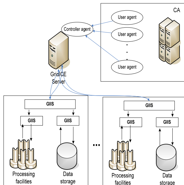
Fig. 9. The interaction of agents with the system
