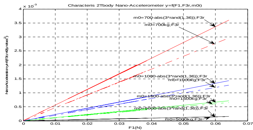
Fig. 8. Nano-accelerometer characteristics with the function y_s=f(F_1, F_{3r}, m_0)
