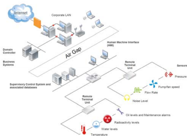
Fig. 2. SCADA network
