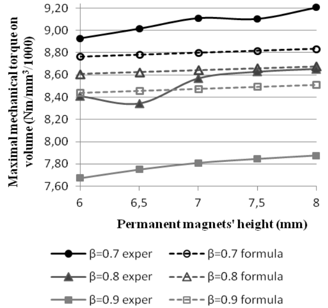
Fig. 6. The function M_{\max}=f(h, \beta) ( l = 30 mm).
