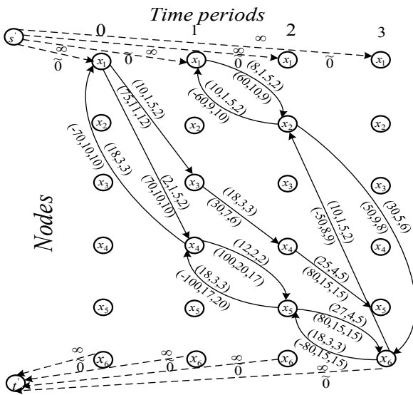
Fig. 5. The residual network \tilde{G}(\tilde{\xi}^\mu(x_i, x_j, \theta, \theta)) for the graph \tilde{G}(\tilde{\xi})
