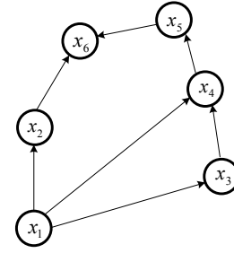
Fig. 1. Initial dynamic graph \tilde{G}
