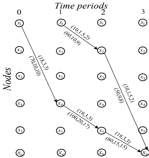
Fig. 4. Graph with the feasible flow \tilde{G}(\tilde{\xi})
