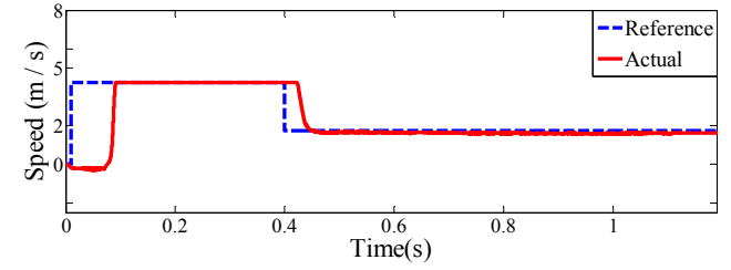
Fig. 5. Speed reference signal and speed actual of the motor by the proposed sliding mode observer.
