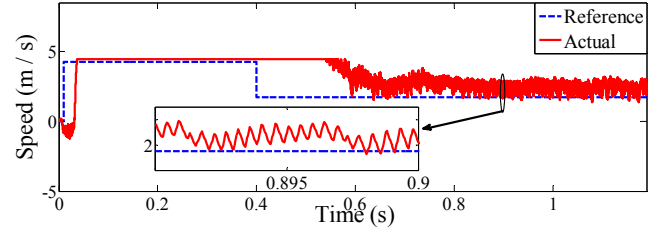
Fig. 4. Speed reference signal and actual speed of the motor by sliding mode observer.
