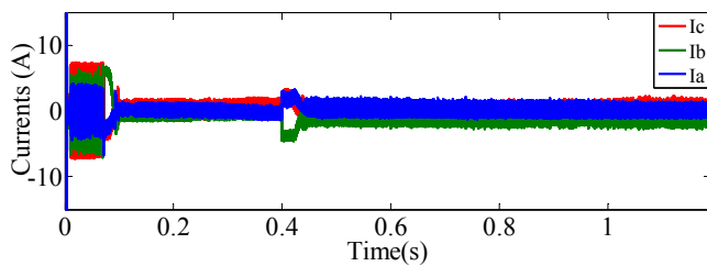
Fig. 8. The currents of PMLSM which uses the proposed sliding mode observer.
