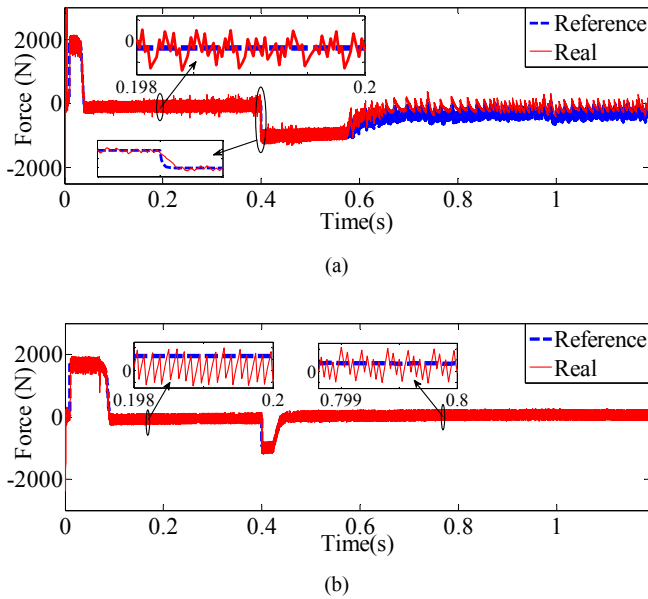
Fig. 7. The produced force of the mover (a) by using a conventional sliding mode observer (b) by using the proposed sliding mode observer.
