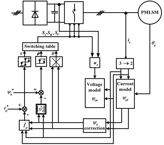
Fig. 1. DTFC block diagram.
