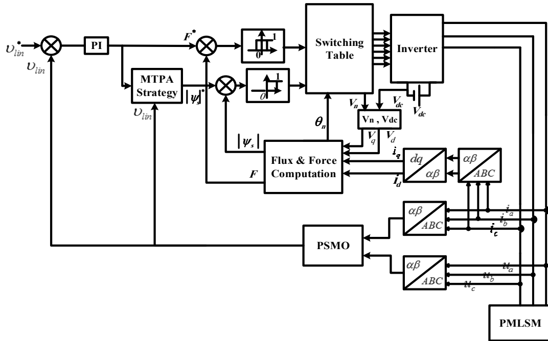
Fig. 2. Block diagram of the PMLSM sensorless control.
