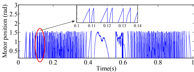
Fig. 9. Position response for the motor.
