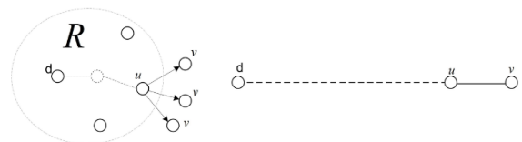
Fig. 4. Applying Dijkstra's algorithm.
