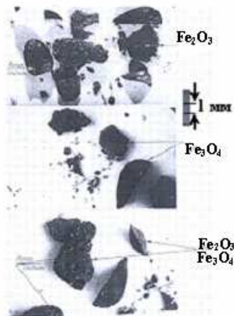
Fig.4. Structure of the thermite.
