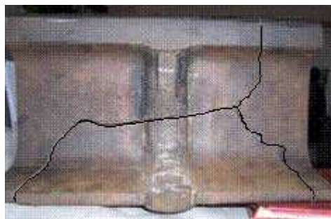
Fig.1. View of a thermic weld fracture
