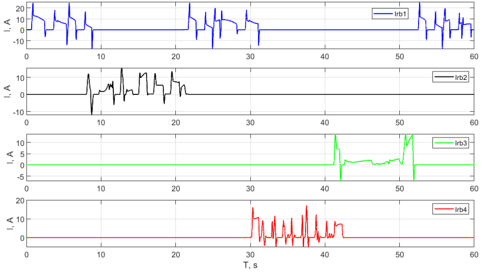
Fig. 3.26. Example of a 60-second repetitive industrial production cycle and consumer electrical load current profiles in the case of four industrial robots assisting for several operations: IRB1 – material handling; IRB2 – to carry a welding gun; IRB3 – to carry a glue dispenser; IRB4 – to carry clinching equipment.
