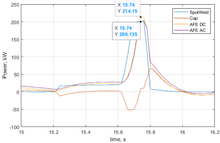
Fig. 4.6. Spot welding instance power of spot welding tool, active front-end AC and DC side and capacitor module.
