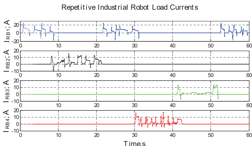
Fig. 1. Example of 60 second repetitive industrial production cycle and consumer electrical load current profiles in case of 4 industrial robots assisting for several operations: I_{RB1} – material handling ; I_{RB2} – carry welding gun ; I_{RB3} – carry glue dispenser ; I_{RB4} – carry clinching equipment.
