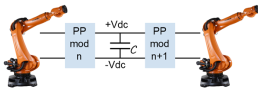
Fig. 1. Energy saving system and PP modules.
