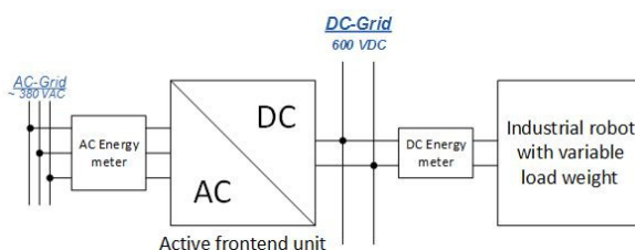
Fig. 2. Principal electrical schematic of the experimental setup.
