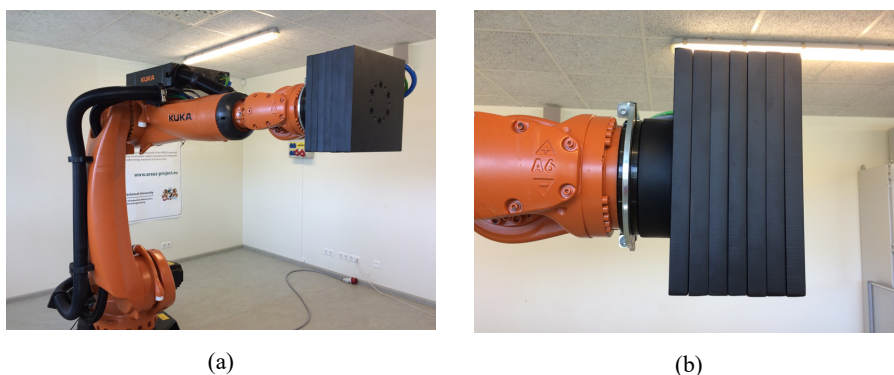
Fig. 1. Whole industrial robot arm with load (a); variable load (b).
