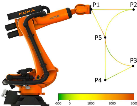
Fig. 6. Programmed trajectory with the power consumption data
