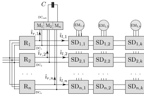
Fig.1. Block diagram of DC subgrid for energy exchange.
