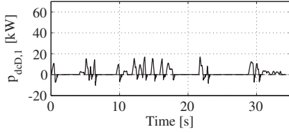
Fig. 2. Consumption of a single robot, k = 1
