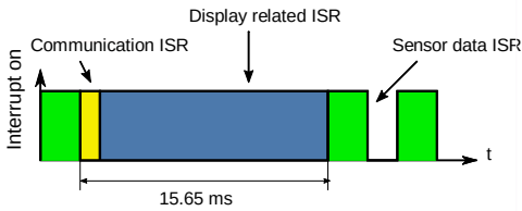
Fig. 11 Delay introduced by display related ISR.
