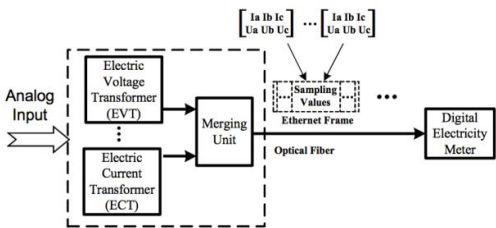
Fig 1. Electrical Energy Measurement in Digital Substations[4].
