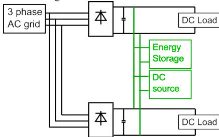
Fig. 1. General overview of electrical system representing conventional power system in black and optional connections for element integration in DC network in green
