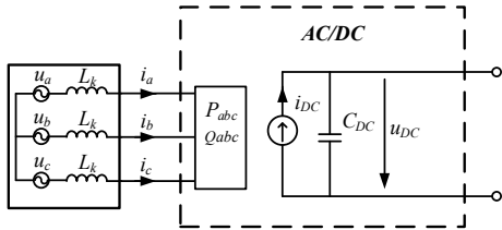
Fig. 2. Model structure of AC/DC converter.
