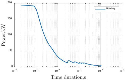
Fig. 6 Power analysis results of welding power profile.
