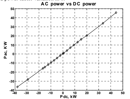
Fig. 3. AC side power with respect to DC side power.
