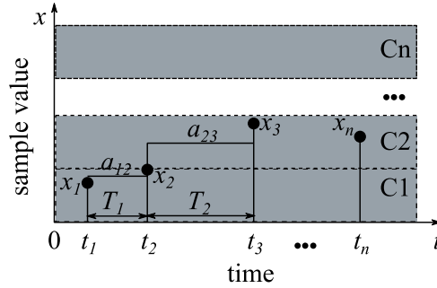
Fig. 3.28. Graphical representation of current sample x categorization analysis within classes C .
