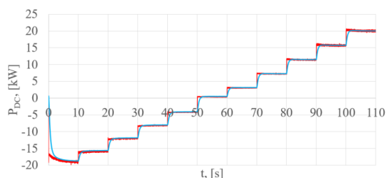
Fig. 11. The second case: constant power steps throughout the motor drive system's power range. Measurements from the novel DC power meter (red line) and the N4L PPA5530 power analyzer (blue line).
