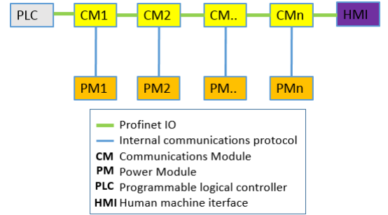
Fig. 9. Line structure of Profinet IO network.
