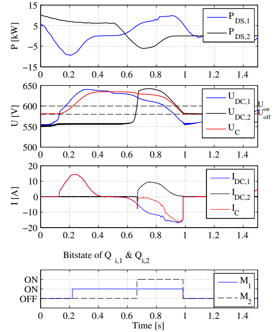
Fig. 6. Simulation of energy exchange between drive systems and asynchronous switching at voltage control levels: 580 V and U_{on} 600 V, allowed voltage difference for coupling U_{\Delta} \leq 20V .
