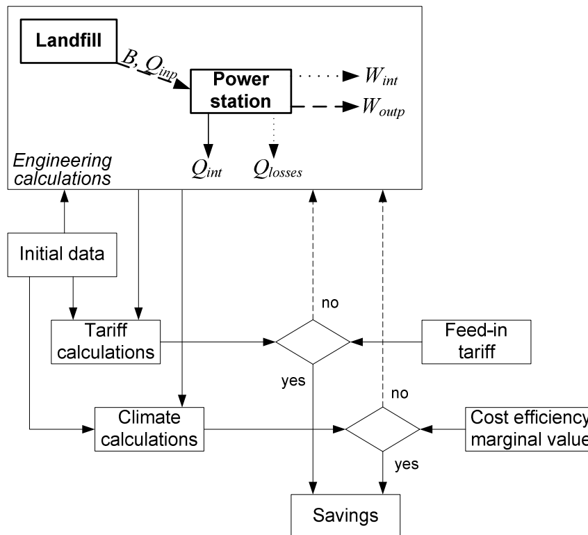
Fig.1. Calculation model for landfill biogas power station
