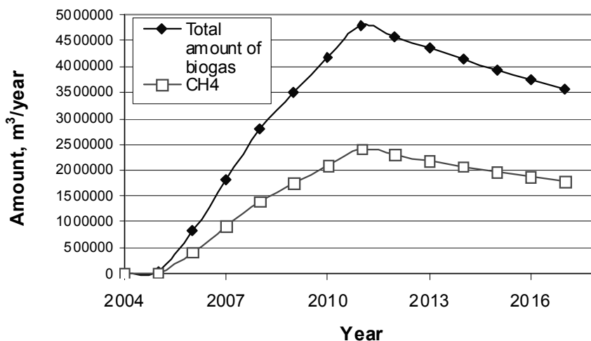
Fig.3. The amount of biogas produced at landfill “Daibe”
