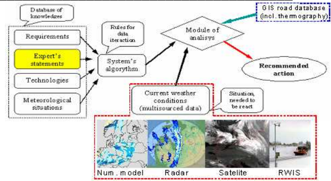
Fig.2. Architecture of expert system's prototype for winter road maintenance
