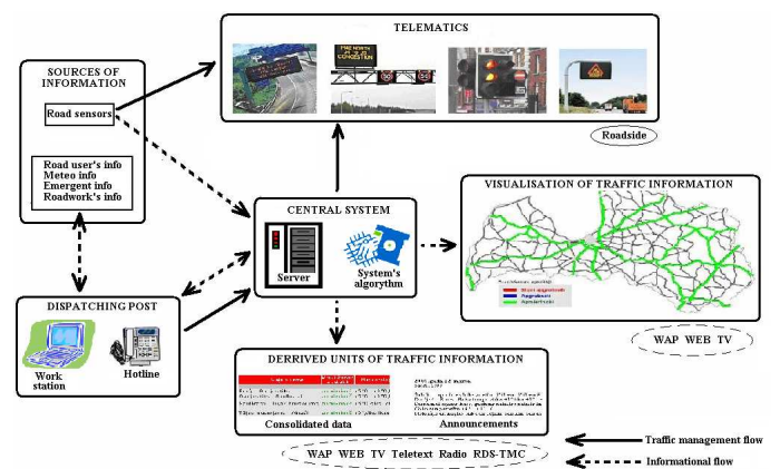
Fig.4. Functional data flows in ITS structure
