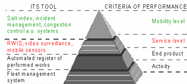
Fig.10. ITS solutions for different tasks of road winter maintenance
